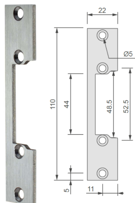
Bouts carrés - 110 x 22 mm
